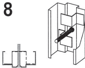
8 PUNCH & DIMPLE 3/8" BOLT B.O.
