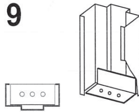
9 FLOOR ANCHOR
