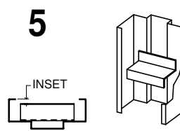
ZEE ANCHOR INSET
